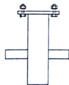
80 120MM BORE SIZE 4 7MM THICKNESS PIPE, ROUND PLATE: 250MM DIA WITH 10MM THICKNESS
